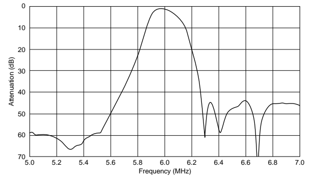
SFSRA6M00BF00-B0
