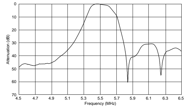
SFSRA5M50CF00-B0
