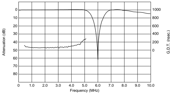
TPSKA6M00B00-R1
