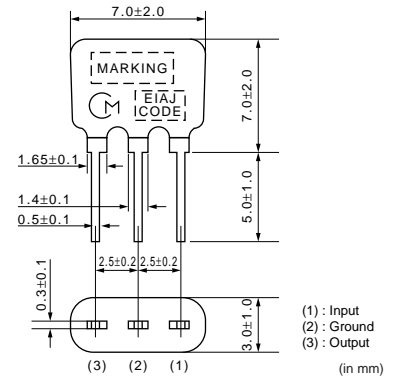
SFVLF10M7MF00-B0
