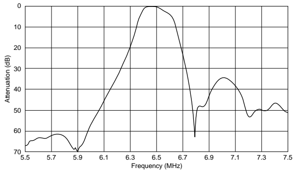
SFSRA6M50BF00-B0
