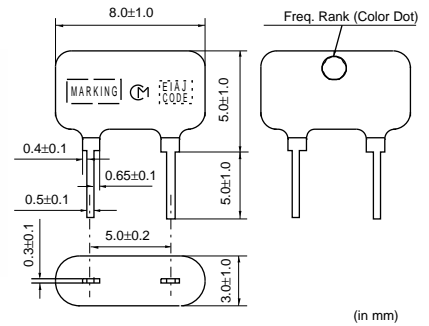
CDALF10M7C_Series
