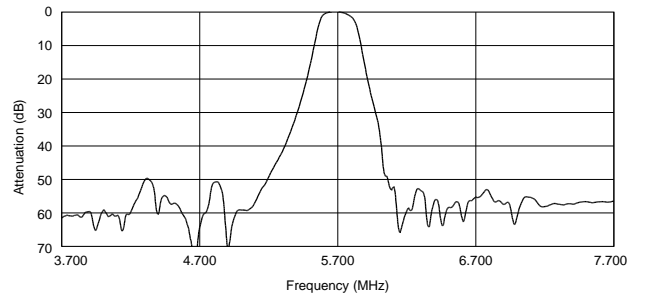
SFSKB5M70GF00-R1
