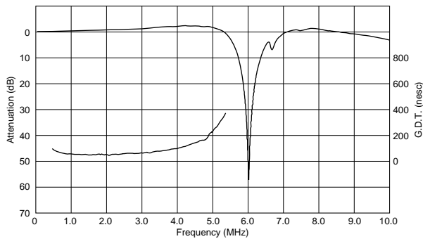
TPSRA6M00B00-B0
