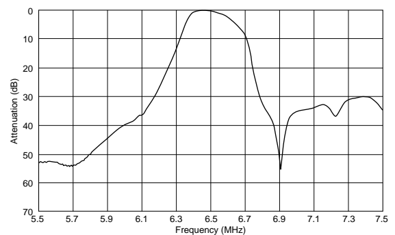
SFSRA6M50CF00-B0
